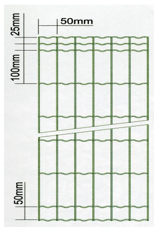
Eurofence Plus (2,2 mm) Eurofence strong (2,5 mm)
